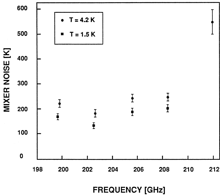
Fig.16 Mixer noise temperature versus frequency at two physical temperatures: 1.5K and 4.2K.
