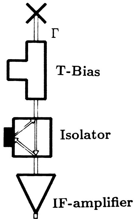
Schematic Diagram of junction and IF-chain
