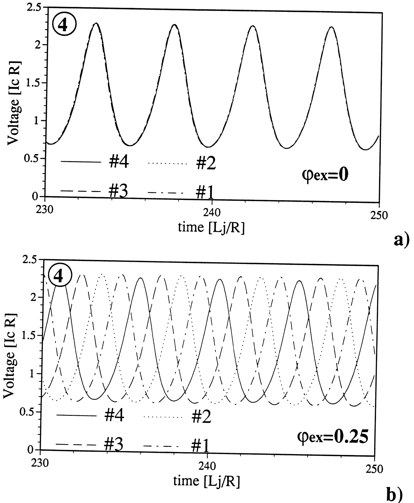
Figure 7. The waveforms of individual junction voltages for the in-phase state labeled "4" in Fig. 5. a) No DC magnetic field supplied. b) Quarter of the flux quantum in every loop supplied by the external magnetic field. Voltage waveforms uniformly shifted by quarter of a period. The main beam of the radiation is steered from the broadside direction.
