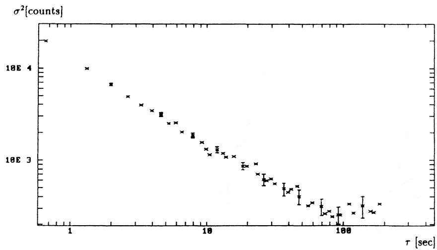
Allan plot
