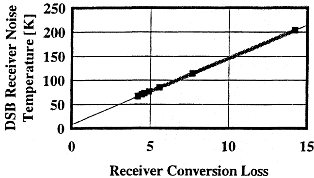
Figure 5. Receiver DSB noise temperature versus conversion loss measured at the different levels of the local oscillator power. Experimental points are located on a strait line.
