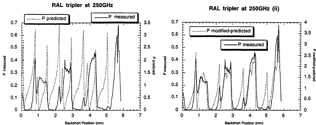
Figure 9. Comparison of measured tripler performance and prediction using phase-modified embedding impedance.
