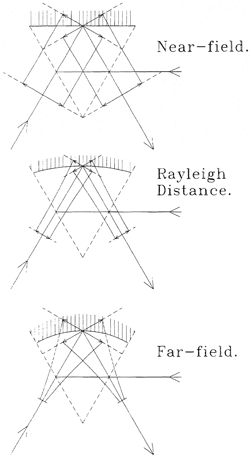
Figure 3: Quasi-optical beam trajectories in a triangular FFP for f = 6 GHz and f = 800 GHz. The pictures are an illustration of the values in Table II.
