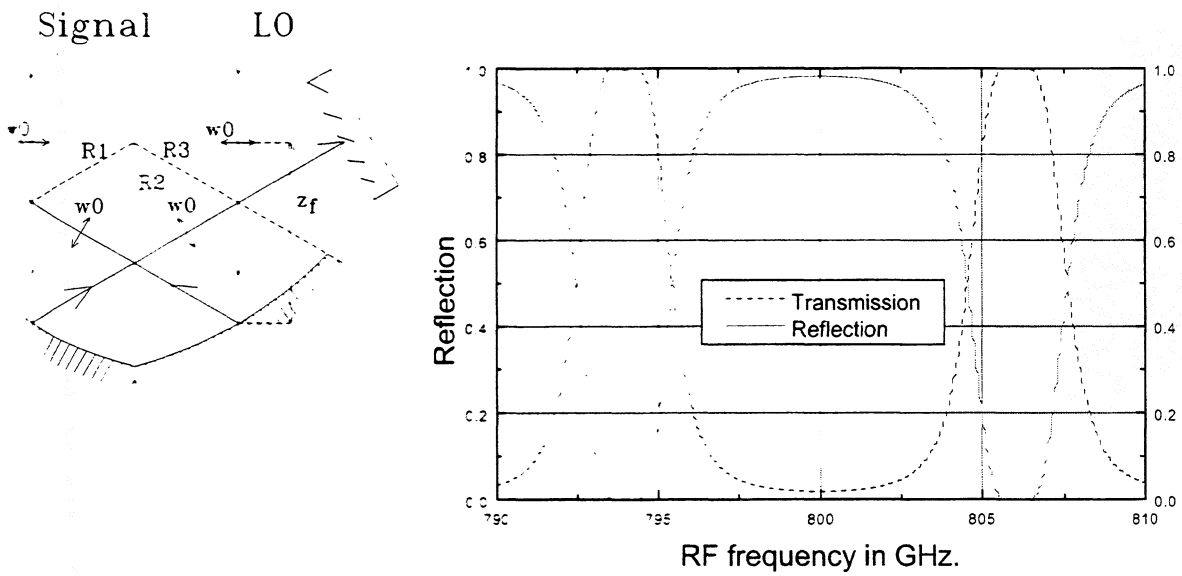
Figure 6: Configuration with 2 triangular FFPs in series. Transmission is calculated for R1 = R3 = 0.243 and R2 = 0.664 .
