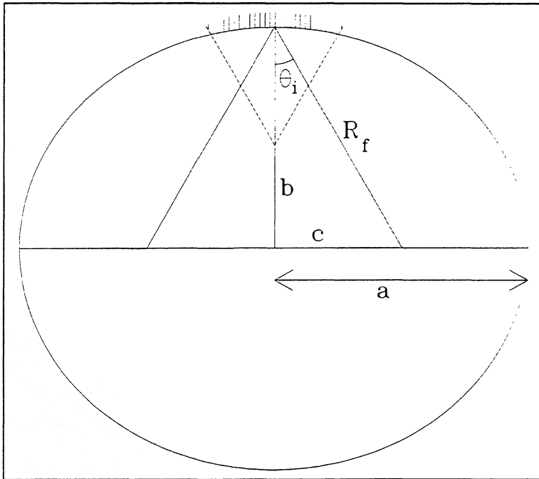
Figure 4a: Geometry of the elliptical reflector in a triangular FFP with \theta_i = 30^\circ .
