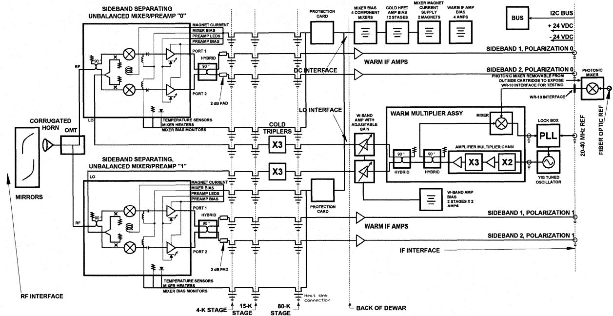
Fig. 1. Block diagram of cartridge.
