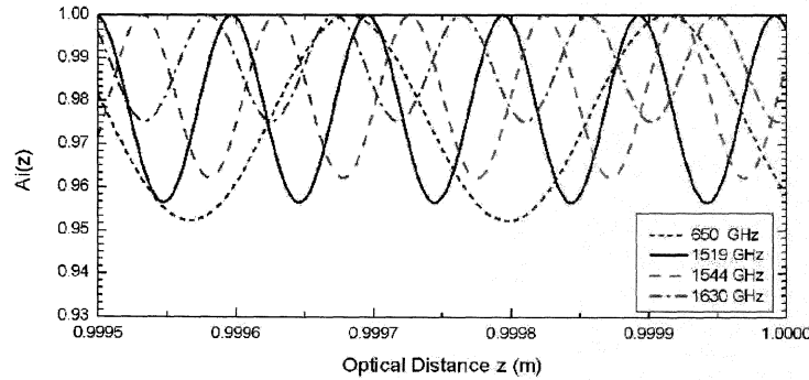
Fig. 1. Standing wave ( A(z) ) for a cavity path length of z=1 meter. Note the effect of atmospheric loss (damping) on the standing wave. Shown here are the last 500 \mu\text{m} . In the example |r_m|^2 was taken to be 0.10 (-10 dB), |r_{lo}|^2 0.16 (-8 dB), and |r_{bs}|^2 0.10(-10 dB) for all four frequencies shown. If there were no atmospheric loss (space, or a high dry mountain site), the peak-to-peak standing wave amplitude in the example would be 4.934%. Solid curve is for \nu_{lo}=1.519 THz, dashed 1.544 THz, dash-dot 1.630 THz, and dotted 650 GHz. We include 650 GHz as a reference where the loss is taken to be 4x less than at 1544 THz. At this frequency SIS receivers in the laboratory are known to be stable to 100 seconds in a 1 MHz resolution bandwidth[5].
