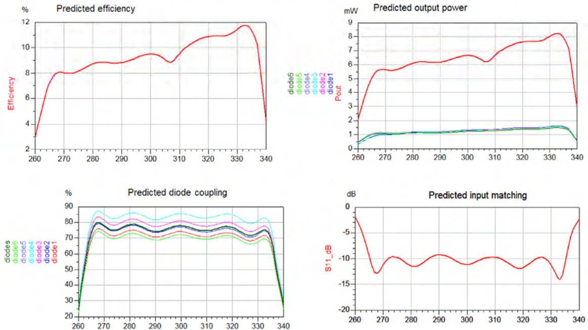
Fig. 4: Predicted performance of the 6-anode 260-340GHz balanced tripler at room temperature with 70 mW of input power. When cooled to around 120K the conversion efficiency of the multiplier is expected to reach 20% at 300 GHz. The coupling at the input frequency is calculated for each diode (left and bottom curves). The calculated output power per diode is shown on the right and top curves along with the total output power.
