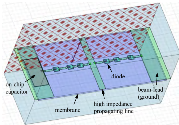
Fig. 2: diode cell used to optimize the channel cross-section dimensions, the location of the 6 anodes and the air-bridge size. One of the HFSS ports is shown in the back side of the diode cell.
