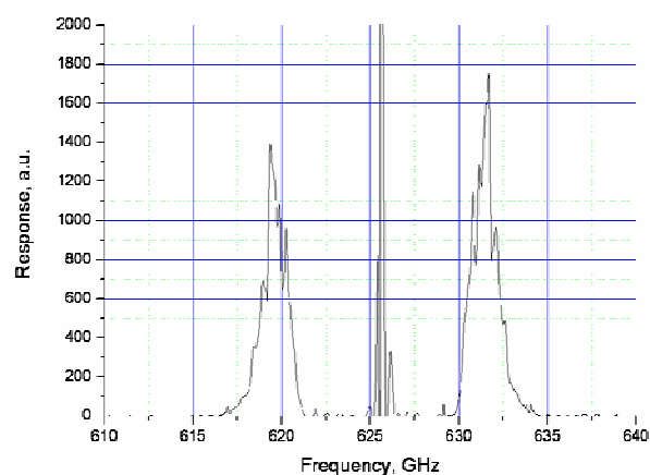
Fig. 12 FTS spectrum of the receiver. LO frequency is 626 GHz. Two sidebands of the receiver are mirrored around the LO frequency.
