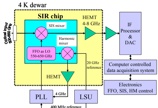
Fig. 5 Schematics of the SIR with a phase-locked LO. The FFO frequency is mixed in the Harmonic Mixer with the 19-21 GHz reference. The mixing product is amplified, down converted and compared with the 400 MHz reference in the PLL. The phase difference signal generated by PLL is used to feedback the FFO control line
