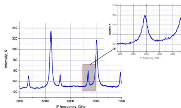
Fig. 11 Deconvolved spectrum of the OCS emission lines at a gas pressure 2.6 mBar. LO frequency 601 GHz. Two strong lines are saturated; weaker lines are not saturated isotopes. The lines are detected, one in the LSB, the other one in the USB
