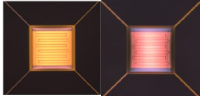
Fig. 7 Photographs of TES detectors with thermally isolating straight legs fabricated from 200 \text{ nm} thick silicon nitride (SiN). The image at the left is a 100 \text{ mm} \times 100 \text{ mm} Mo/Au (yellow) with interdigital Au bars. The image at the right is a 100 \text{ mm} \times 100 \text{ mm} Mo/Cu TES with the same geometry. The width of the legs in the left hand picture is 2 \text{ mm} and the width of the legs in the right hand picture is 4 \text{ mm} . Both have legs with length 420 \text{ mm} .
