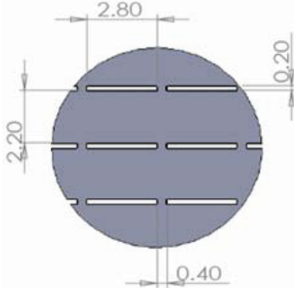
Fig. 4 Geometry of rectangular element
