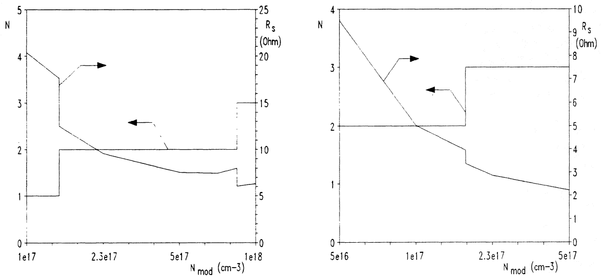
Fig. 8. The same as Fig. 6, but for GaAs/GaN.
