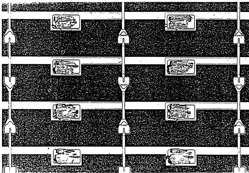
Figure 4: Photograph of a small section of the beam control array. Unit cell dimensions are 300\ \mu\text{m} \times 120\ \mu\text{m} . The vertical strips serve as the “antenna” elements, while the horizontal strips provide bias voltage to the diodes. The marks on the large rectangular test pads are from automated device probing.
