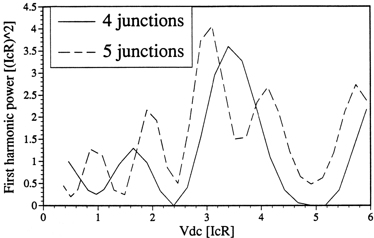
Figure 9. Comparison between the 4-junction and 5-junction small inductance arrays; \lambda = \pi/5 , \beta = 0.03 . As the number of junctions increase, more maximums and minimums appear throughout the operating range.
