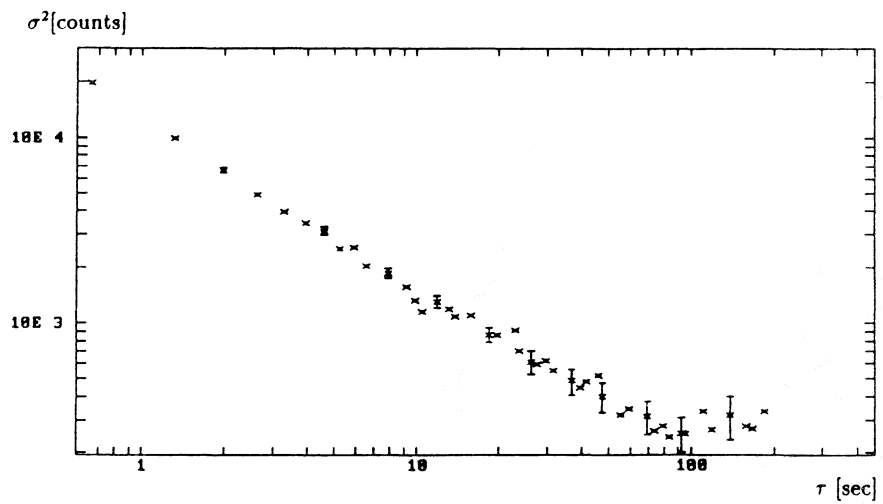
Allan plot
