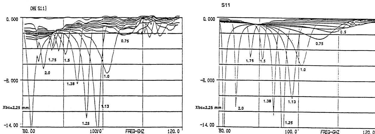
Figure 1. Comparison of measured and computed values for the return loss between the embedding circuit and a 50Ω junction. Frequencies have been scaled to the 3mm range.
