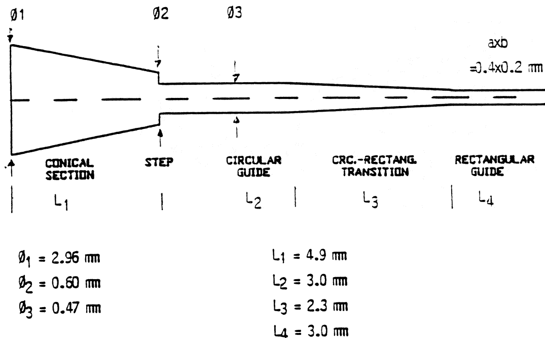
Fig. 3: DUAL - MODE HORN (SCHEMATIC)
