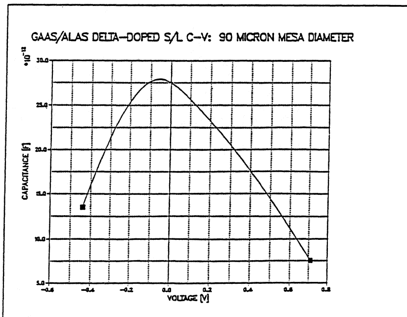
FIGURE (8): Structure III: C-V characteristic
