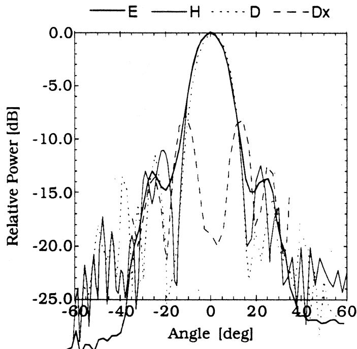
Fig. 3c. Antenna patterns for the BLTSA designed for the 348 GHz design measured at 802 GHz
