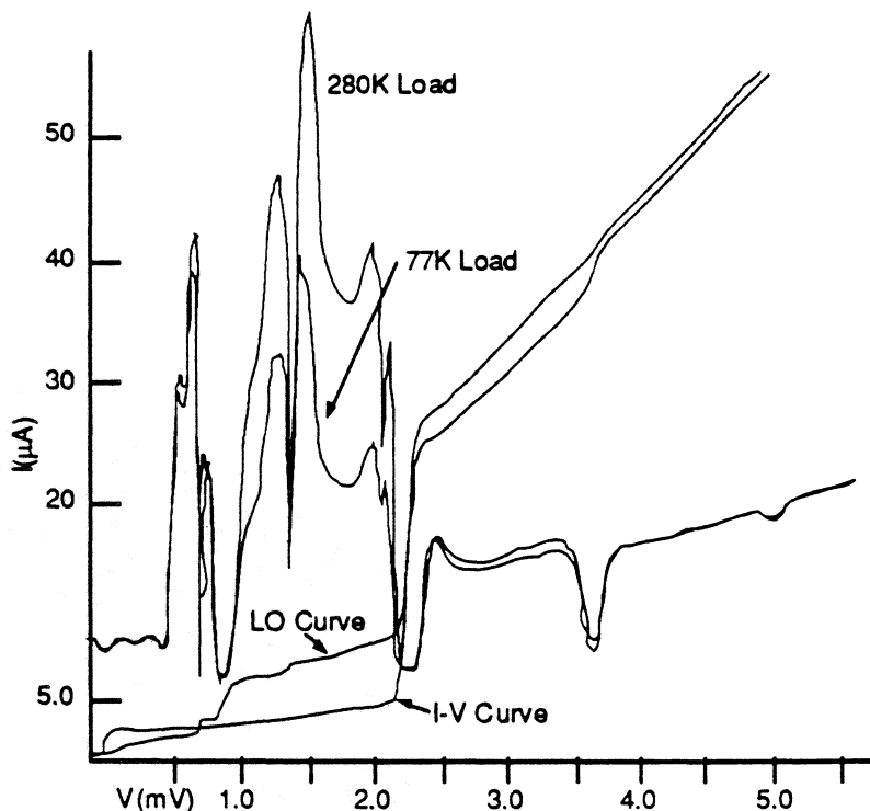
JUNCTION I/V & IF POWER CURVES WITH REDUCED MAGNETIC FIELD
