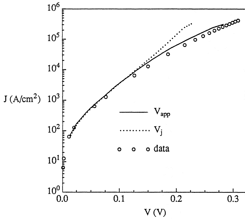
Figure 5a. Forward current-voltage characteristic of In 0.5 Ga 0.5 As/InP Schottky diode.
