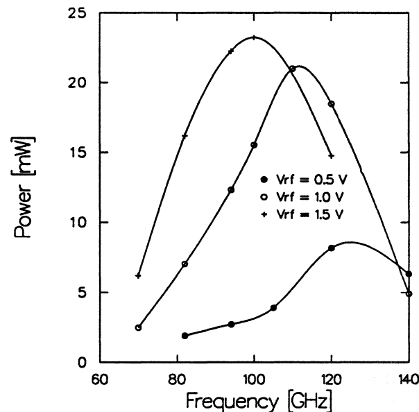
Figure 3: Power vs. frequency for a 1.7 \mu\text{m} long InP Gunn device doped at 9 \times 10^{15} \text{ cm}^{-3} . Diameter = 40 \mu\text{m} , V_{\text{dc}} = 4.0 \text{ V} , T = 450 \text{ K} .
