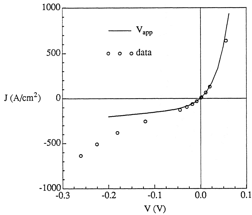
Figure 5b. Reverse current-voltage characteristic of In 0.5 Ga 0.5 As/InP Schottky diode.
