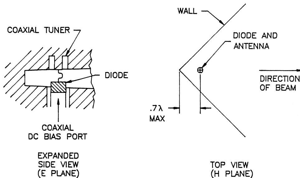
Fig. 1. Top view and side view cross section of the quasi-waveguide tripler.
