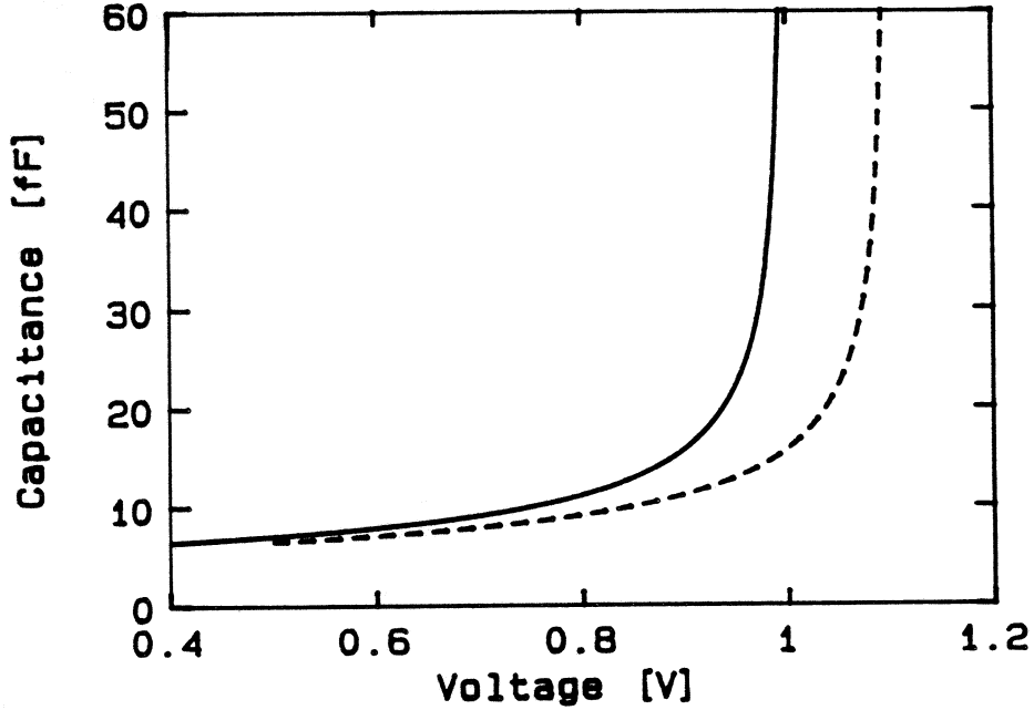
Figure 2: The junction capacitance at temperatures 300 K (solid line) and at 77 K (dashed line).
