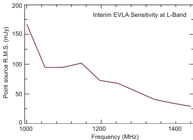
Figure 3. The point source rms values for L-Band frequencies between 1000 and 1440 MHz.
