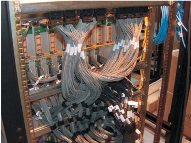
Figure 1. High speed data cables installed in a WIDAR station rack.
