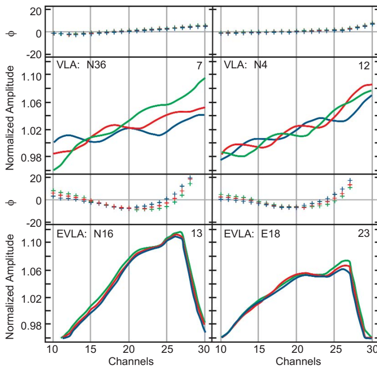
Figure 1. Normalized amplitude and phase bandpass solutions for VLA Antennas 7 and 12 (top panels) and EVLA Antennas 13 and 23 (bottom panels), for three observing frequencies: 8448 MHz (green), 8450 MHz (blue), and 8452 MHz (red). In each case the total observing bandwidth is 12.5 MHz.
