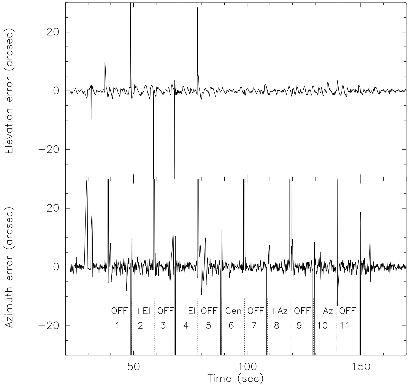
Vertex antenna: motions during FivePoint scan
