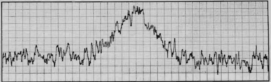
VENUS PASSING THROUGH BEAM OF EWEN KNIGHT RADIO TELESCOPE Bulges mean more than wiggles.
