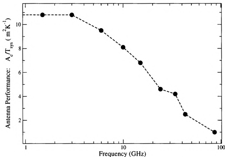
Figure 4.1: The required antenna sensitivity parameter, A_e/T_{sys} , for the NMArray antennas. The requirements refer to the band centers, marked by the filled circles. The dashed line is provided only for continuity. Degradation in performance up to 10% at the band edges is permitted. A greater degradation at the low end of the 1 – 2 GHz band is expected.
