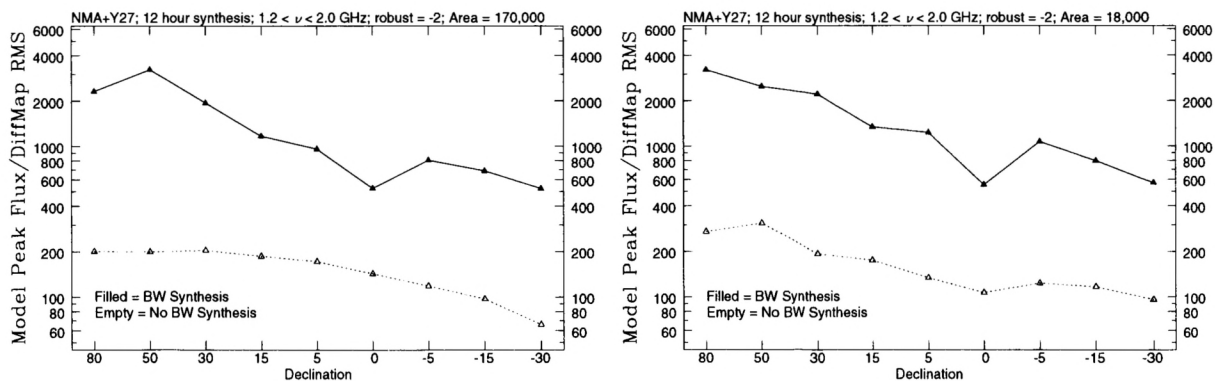
Figure 5.3: Anticipated imaging fidelity for large and complex sources with the full-resolution EVLA. The methodology of the simulations is described in the text. In the left panel, the trial source is 170,000 times the solid angle of the synthesized beam. In the right panel, it is 18,000 synthesized beams. For each simulation, the ‘dip’ at \delta = 0^\circ is due to the horizontal loci of the u, v tracks.
