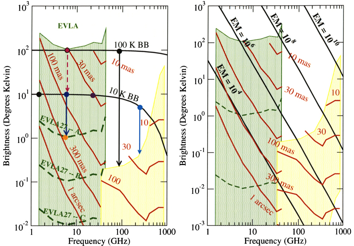
Figure C.1: The continuum brightness temperature sensitivity ( 1-\sigma in 1 hour) of the EVLA (shaded green) and ALMA (shaded yellow), as a function of frequency and resolution. The brightness temperatures of 10 and 100 K blackbody emission are overlaid in black in the left panel. In the right panel are overlaid the apparent brightness temperature of 10^4 K HII regions with emission measures (EM) from 10^4 to 10^{10} \text{pccm}^{-6} . The array resolutions are shown in red. The upper boundary for each instrument is set by its brightness sensitivity at full resolution. A source can be resolved (at 1-\sigma in 1 hour) at the resolution given by the red lines if the source brightness (shown by the appropriate black line) lies within a shaded area. Refer to the text for a more comprehensive description.
