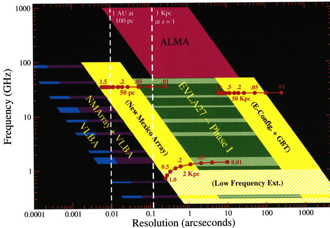
Figure 2.4: The frequency-resolution coverage after completion of the EVLA (Phase I in green, and Phase II in yellow) and ALMA projects, plus the incorporation of the VLBA into the EVLA. Phase II of the Expanded VLA Project will greatly increase the ‘Discovery Space’ area available to NRAO telescopes. The regions opened by each of the two components of Phase II are shown in yellow. The hashed yellow portion is the coverage available with a subsequent expansion of the low frequency capability. The ‘evolution lines’ from the last figure are reproduced, showing that combining the E-configuration and the GBT will allow imaging of 50 kpc structures as close as z = .025 , and that 50 pc-scale emission will be resolved anywhere in the Universe with the addition of the New Mexico Array.
