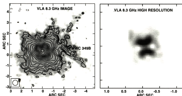
Figure B.14: VLA images of the thermal stellar-wind source MWC 349, a B[e] star. The left panel shows a naturally-weighted image intended to emphasize weaker features: in addition to the thermal emission from MWC 349 itself, a weak bow shock is seen at the location of the interaction with the wind of a B star companion, MWC 349B. The right panel shows a super-resolved MEM deconvolution, giving high spatial resolution in areas of strong flux (data from Rodríguez & Bastian 1994; courtesy S. White 1999).
