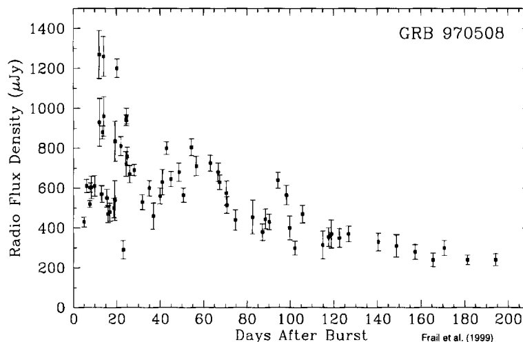
Figure 3.19: 8.5GHz light curve of the radio afterglow from GRB 970508 (Frail et al. 1999). The flux density fluctuations at early times are the result of refractive interstellar scintillation, an interference effect produced by the intervening ionized gas along the line of sight. This scintillation provides a direct measurement of the angular size of the expanding fireball, and the only direct observational evidence that these sources and their afterglows are relativistic shocks. At late times ( > 100 days) the radio light curve undergoes the same power-law decay seen at X-ray and optical wavelengths. When the GRB itself has faded from view, the NMArray will provide images and accurate astrometry of the host galaxy, yielding precise position offsets even for those ‘dark’ GRBs whose optical emission is either intrinsically faint, or obscured by dust.
