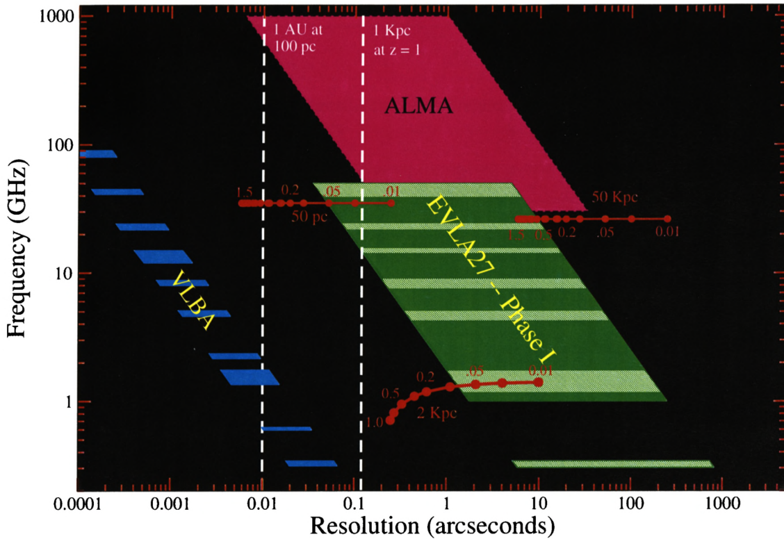
Figure 2.3: The frequency-resolution coverage after Phase I of the EVLA is shown in green, along with coverage by the VLBA and ALMA. The area covered by the EVLA will more than double that of the original VLA, shown within the narrow horizontal bands in light green. The vertical dashed lines show the angular size of an object of 1 AU in extent at the distance of 100 pc, and the angular size of a 1 kpc source at z = 1 . The superposed red traces are ‘evolution plots.’ The lowest one shows the locus of observed frequency and angular size of H I emission from a 2 kpc object between z = 0.01 and z = 1 . The present VLA cannot detect, or resolve, such an object in H I emission beyond z = 0.1 . The upper traces show the evolution of the angular size of a 50 pc object (left) and a 50 kpc object (right) as a function of redshift between 0.01 and 30 (the minimum angular size occurs at z = 1.6 ). For these two examples, it is assumed the observations are made at a fixed frequency, so the frequency shift is not shown. A flat cosmology, with \Omega_m = 0.27 and H_o = 71 \text{ km s}^{-1} \text{ Mpc}^{-1} , is assumed.
