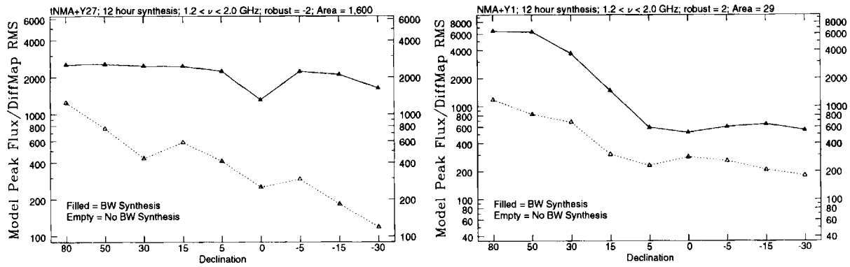
Figure 5.4: The left panel shows the fidelity when the EVLA data are tapered to a resolution one-third of the maximum. The source is the same angular size as the right hand panel simulation in Fig. 5.3, but because the array has been tapered, the number of resolution elements in the trial object is reduced to 1600. In the right panel is shown the fidelity of the New Mexico Array plus one VLA antenna to a trial source whose solid angle is 29 synthesized beams.
