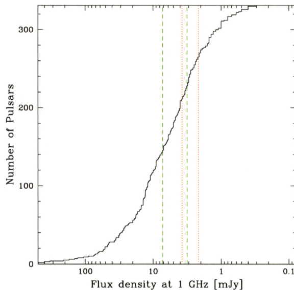
Figure B.17: Cumulative distribution of pulsar flux densities. The vertical lines indicate flux density limits for two different parallax estimates: the dashed green lines show pulsars whose distances could be measured if they were as far away as 8 kpc, while the dotted red lines show those which could be measured out to 3 kpc. The two lines in each case correspond to the range of measured spectral indices ( \nu^{-1.4} - \nu^{-2.4} ).
