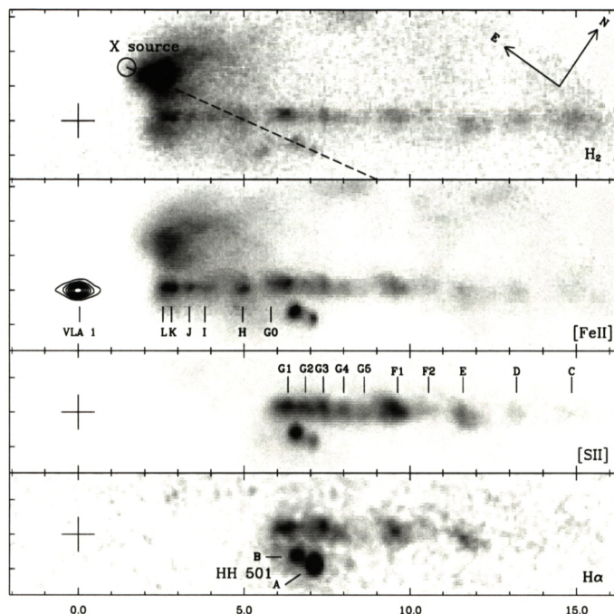
Figure B.5: The thermal jet in HH 1–2, combining VLA 8.4 GHz ( contours ) with HST optical and near-IR ( grayscale ) data. The [Fe II] panel in particular shows the radio emission from the thermal jet (VLA 1) extending about an arcsecond, while the [Fe II] picks up several arcseconds out and extends to \sim 10 arcseconds. The NMArray will give at least a factor 10 higher resolution as well as filling in the missing emission, allowing us to follow the jet continuously from the origin to the working surface (the Herbig-Haro objects). Courtesy L. Rodríguez, based on Reipurth et al. (2000).
