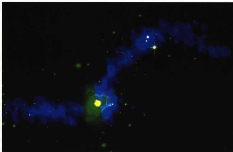
Figure B.26: A composite image of the optical light (green), star forming regions (yellow and pink), and cold atomic hydrogen gas (blue) in the well known merger remnant NGC 7252, the "Atoms for Peace" galaxy. The name derives from the pair of tidal tails and the loops surrounding the optical body. This system is the result of the merger of two spiral galaxies. The H I data show that the tidal tails are rich in gas, confirming the gas-rich nature of the progenitor disks. They also show that the inner regions are relatively free of cold atomic gas. These data support the idea that merging spirals can create gas-poor elliptical galaxies. From Hibbard et al. (1994).
