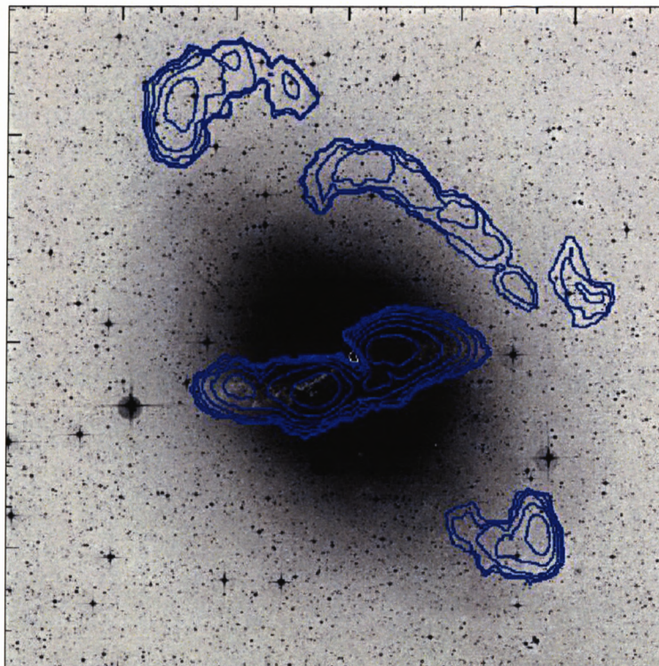
Figure B.25: Neutral hydrogen contours atop optical grayscale for the E/S0 galaxy NGC 5128 (Centaurus A). The H I distribution follows and is slightly displaced from the outermost diffuse shells. From Schiminovich et al. (1994).
