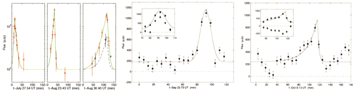
Figure B.16: Radio emission from three brown dwarfs, as observed with the VLA: (left) LP 944–20; (middle) TVLM 513–46546; (right) 2MASS J0096159+182110. The insets show the circularly polarized flux density ( \sim 60\% ). The sensitivity of the EVLA combined with the resolution of the New Mexico Array will allow sub-stellar astrometric measurements of both the quiescent and the flaring emission, providing direct measurements of changes with rotation and orbital phase, offsets between the flares and the normal emission, etc. From Berger et al. (2001) and Berger (2002).
