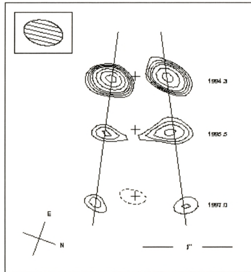
Figure B.7: Difference maps of the thermal radio jet in the HH 80–81 complex for the epochs 1994.3–1990.2, 1995.5–1990.2, and 1997.0–1990.2. Crosses indicate the position of the central source. The corresponding outflow velocity is \sim 500 km/sec, with ejection occurring about every 10 years. From Martí et al. (1998).
