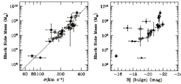
Figure 3.7: The mass of supermassive black holes in galactic nuclei, vs. central velocity dispersion ( left ) and bulge B -band luminosity ( right ). The tight correlation indicates a fundamental connection between the evolution of black holes and their host galaxies. From Ferrarese (2002).
