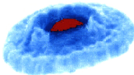
Figure B.2: A three-dimensional reconstruction of Jupiter's synchrotron radiation at 1.4 GHz, based on data taken with the VLA and the ATCA. The red circle represents the planetary surface. From Sault et al. 1997; de Pater & Sault 1998; and Santos-Costa et al. 2001; see http://www.atnf.csiro.au/research/solarsys/jupiter/movies/ for the full movie.
