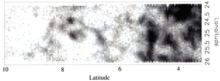
Figure B.22: The Galactic H I emission measured by the Green Bank Telescope in the region ( 24^\circ \leq l \leq 26^\circ , 2^\circ \leq b \leq 10^\circ ), averaged over LSR velocities 122–138 km/sec (Lockman 2002). Galactic rotation is expected to give a velocity of \sim 110 km/sec at these longitudes, so this emission must arise close to the tangent point: i.e. , 7 kpc from the Sun. The two halo clouds at b = 7.6^\circ are thus more than 1 kpc above the Galactic plane.
