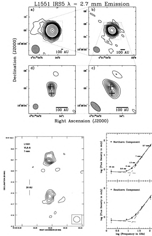
Figure B.8: Dust emission from L1551 IRS5. ( upper ) BIMA (Berkeley-Illinois-Maryland Array) images at 110 GHz with increasing angular resolution (Looney et al. 1997), showing that L1551 is composed of two circumstellar disks located within a flattened circumbinary structure embedded in an approximately spherical large-scale envelope. ( lower ) VLA images at 43 GHz with 50 milliarcsecond (7 AU) resolution (Rodríguez et al. 1998) clearly resolve the individual dust disks surrounding the members of the proto-binary system. The spectral decomposition shows that the dust dominates the emission – and is optically thick – down to \sim 22 GHz, below which optically-thin free-free emission takes over.
