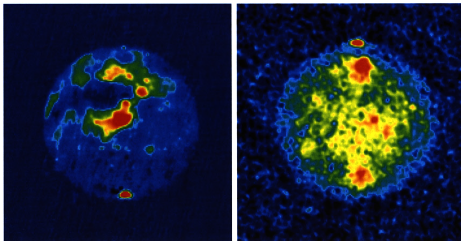
Figure B.1: Radar reflectivity images of Mars ( left ) and Mercury ( right ) made with the combined Goldstone/VLA radar at 4 cm (B.J. Butler, D.O. Muhleman, & M.A. Slade 1999). The EVLA will extend this imaging to much smaller bodies ( e.g. , near earth asteroids and cometary nuclei) and to 13 cm. The latter will probe much deeper into the subsurface than the current 4 cm imaging.
