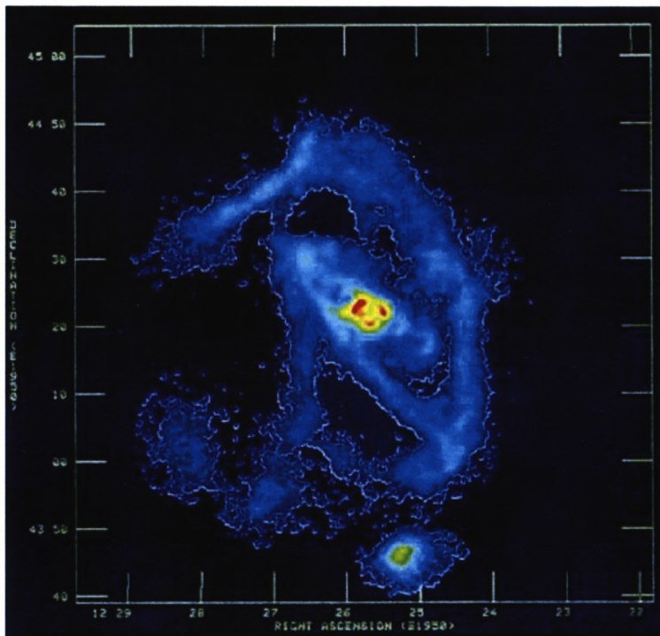
Figure B.24: Pseudo-color representation of the integrated H I distribution of the gas around the dwarf galaxy NGC 4449. This map was made from a mosaic of nine VLA D-configuration pointings plus the pointed map of DDO 125 (the bright object at the bottom edge), and covers more than a square degree. The optical galaxy fits well within the central bright spot in this figure; follow-up observations have found signs of star formation near the peaks of the H I column density, well outside the galaxy. From Hunter et al. (1998).
