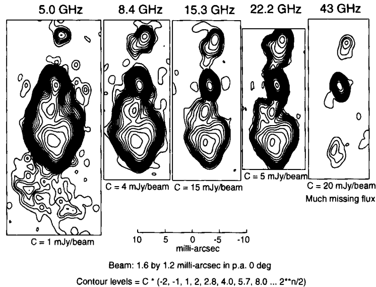
Figure 3.17: Matched-resolution VLBA images of 3C 84 (NGC 1275) from 5 to 43 GHz. Notice the complex spectral structure of the source — the southern extension is seen only at low frequencies, while the northern source gradual elongates towards the nucleus as the frequency increases. This is direct evidence for free-free absorption against the northern lobe; by mapping the spectral index across the source, Walker et al. (2000) were able to derive the parameters of the obscuring disk, including size, scale-height, and rough density distribution. This sort of imaging can be done now only for that handful of sources which happen to fit (at several frequencies) within the very limited spatial dynamic range of the VLBA, and which happen to have turnover frequencies in the correspondingly limited spectral range. This is equivalent to making spectral index maps with only one VLA configuration. Those few sources which have been explored in this way show a variety of structures and scale-heights. The NMArray will provide the intermediate VLA/VLBA spacings needed to extend these measurements to a much wider variety of sources.
