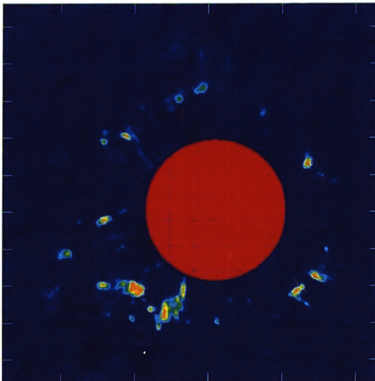
Figure B.13: VLBA image of the star TX Cam, showing the 43 GHz SiO masers forming a shell around the star (Kemball & Diamond 1997). The approximate size of the star is shown by the red circle. Multiple epochs provide direct determinations of the wind outflow speed; simultaneous polarization imaging allows mapping the changing structure of the magnetic field. These observations provide superb resolution but are missing of order half the flux. This missing emission must be more diffuse, and hence should (if imaged with the New Mexico Array) provide much more complete sampling of the atmospheric dynamics and magnetic fields.
