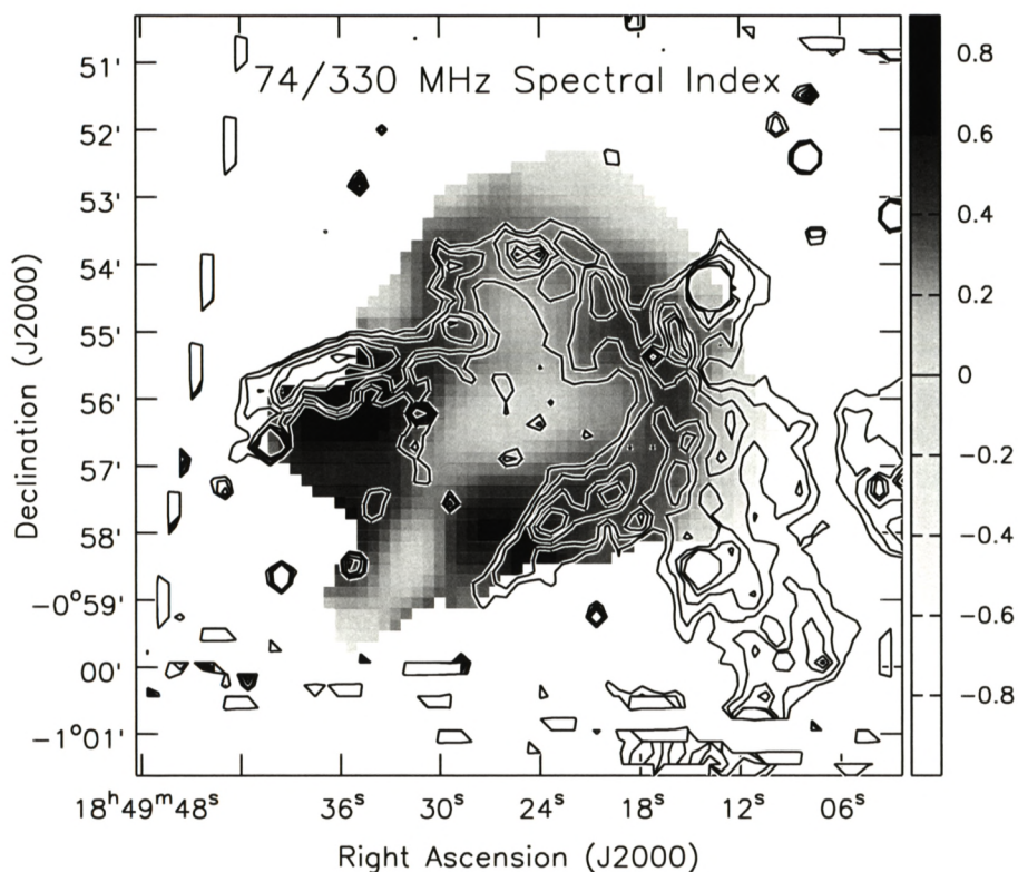
Figure B.18: The supernova remnant (SNR) 3C 391: 74/330 MHz spectral index (grayscale) with ISOCAM 12 – 18 \mu\text{m} contours. Note the impressive agreement between the regions with high spectral index and those with the strongest infrared emission. The spectral index indicates strong free-free absorption, while the bulk of the 12 – 18 \mu\text{m} emission arises from fine structure infrared lines formed in cooling post-shock gas. Both are therefore tracing the SNR/molecular cloud shock boundaries. Courtesy C. Brogan.
