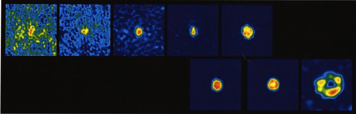
Figure B.15: MERLIN ( upper ) and VLA ( lower ) images of Nova V1974 Cyg 1992 (Pavelin et al. 1993; Hjellming 1996a,b). The 5 GHz MERLIN data were taken 81, 106, 155, 173, and 271 days after outburst; the 22.5 GHz VLA data were taken 255, 313, and 769 days after outburst. Note the evolution from a centered-filled source highly elongated north-south, to a shell slightly elongated east-west. This corresponds to the change from optically thick to optically thin emission, with the later images ‘peeling away’ the outer skin to reveal the three-dimensional structure. The New Mexico Array will have more than 30 times the sensitivity of MERLIN, and (by mapping at 45 GHz) about 10 times higher resolution. Novae like this one could be imaged within a few days of the explosion.
