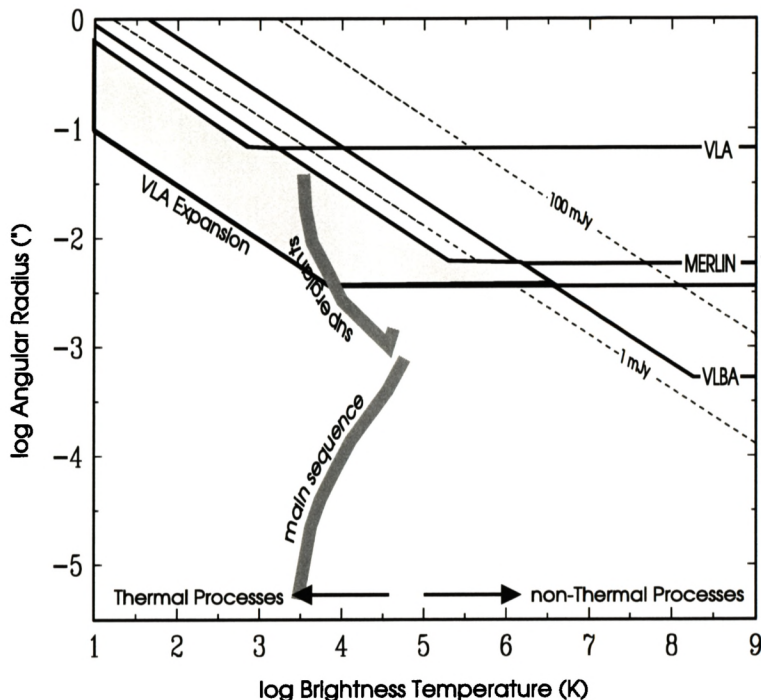
Figure B.9: Brightness temperature and angular size regimes accessible to imaging by interferometer arrays. The previously inaccessible region that will be opened up by an expanded VLA with the upgrade in sensitivity is shown by the shaded area.
