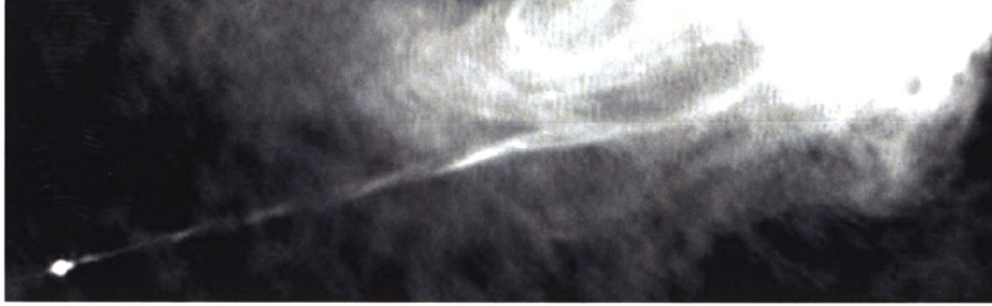
Figure B.28: VLA 4.5 GHz image of the Cygnus A jet, from Perley, Dreher, & Cowan 1984. The jet is only marginally resolved at 0.4'' resolution ( \sim 400\text{pc} at z = .056 ). Helical structure similar to that in M87 can just be seen in this image. Observing with the NMArray at high frequencies will give at least 10 beams across the jet, allowing it to be imaged at a level comparable to the current image of the M87 jet.
