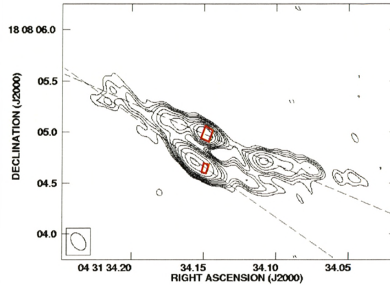
Figure B.6: VLA+Pie Town image of L1551 IRS5 at 8.5 GHz. The half-power beam ( 180 \times 120 mas) is shown in the lower left. The small red rectangles mark the positions and deconvolved dimensions of the compact protoplanetary disks imaged with the VLA at 43 GHz; the dashed lines show the position angles of the jet cores. These data show the jets are already well collimated within 10 AU of the protostars, the most significant constraint yet on jet collimation in young stellar objects. Note too the bends in the jets, which may reflect orbital motions in the binary. From Rodríguez et al. (2003).
