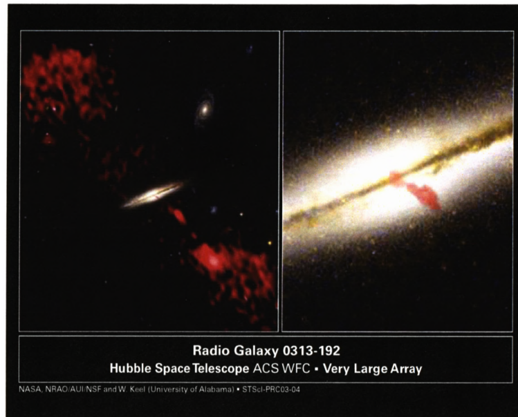
Figure 3.9: The edge-on spiral galaxy 0313–192, as seen at optical (black-and-white; HST) and radio (red; VLA) wavelengths. The optical morphology would suggest that the prime source of energy generation in this system is star formation, but the radio jets and lobes show a substantial AGN contribution. This particular example is both nearby and relatively bright and extended; the NMArray’s combination of sensitivity and spatial resolution will be required to reveal the existence of AGN jets in more distant and typical systems. Image from Keel, Ledlow, & Owen (2003).
