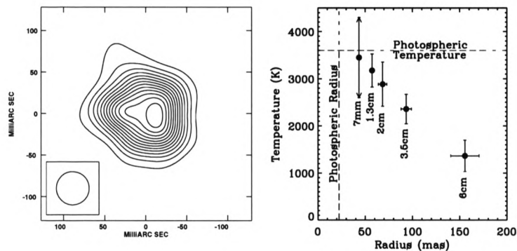
Figure B.10: ( left ) VLA 43 GHz image of Betelgeuse. The resolution is 40 milliarcseconds and the contour interval is 250 K (brightness temperature). ( right ) The variation of temperature in the atmosphere with radius, determined from the VLA observations of Betelgeuse at different frequencies which resolve the source size (Lim et al. 1998). The NMArray will give a factor \sim 10 higher resolution at 30 times higher sensitivity.
