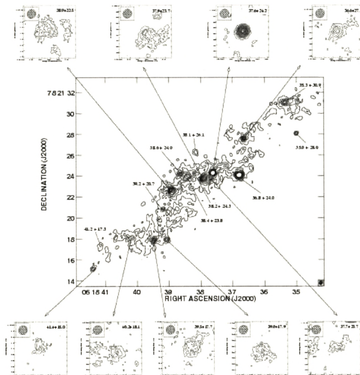
Figure B.23: The starburst galaxy NGC 2146 at 5 GHz, as imaged by combining MERLIN and the VLA's A-configuration (Tarchi et al. 2000). The peak contour in the central image is 640 \mu\text{Jy}/\text{beam} . At a distance of 15 Mpc, only a small fraction of the compact sources are resolved with the 0.15 arcsec beam; some of the unresolved sources are supernova remnants, and some are probably ultra-dense H II regions associated with super star clusters. The sensitivity of the EVLA combined with the long baselines of the New Mexico Array will provide similar signal-to-noise with a 0.03 arcsec beam — just over 2 pc. The H II regions should be at least this strong at higher frequencies, and there the EVLA will allow another order-of-magnitude improvement in resolution.
