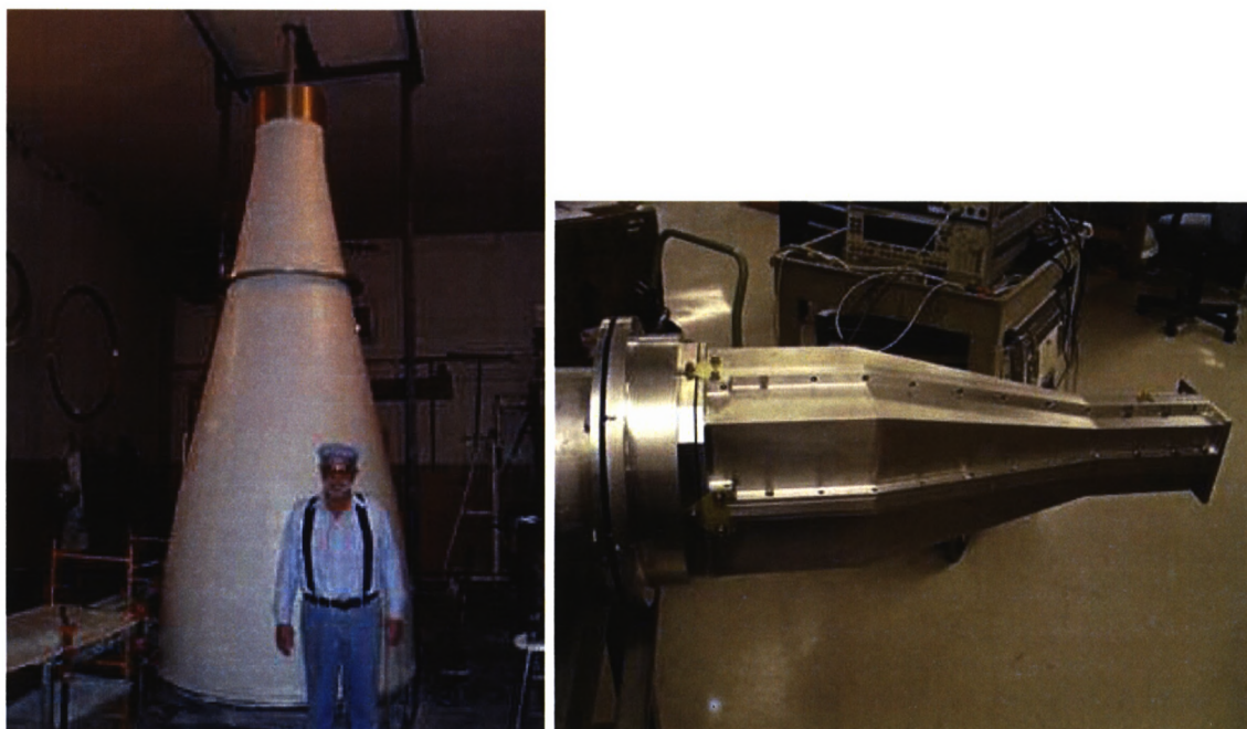
Figure A.2: Prototypes of the 1-2 GHz band feed horn (left) and polarizer (right). These are scheduled to be outfitted on the EVLA test antenna for testing in April 2004.
