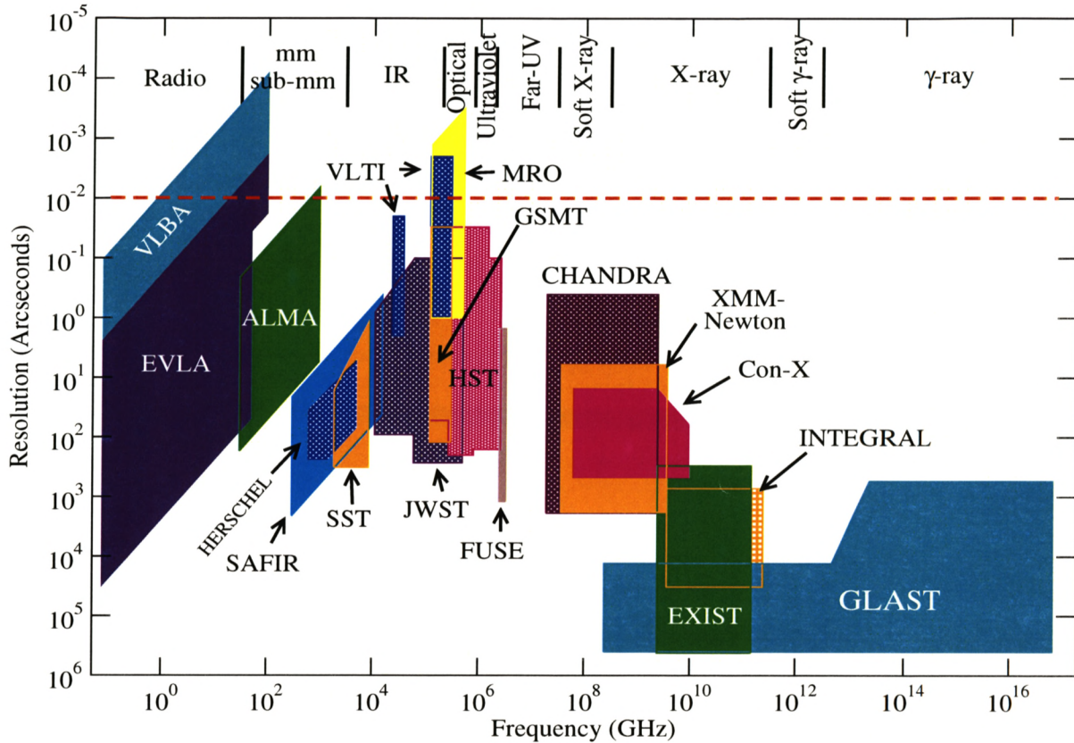
Figure 2.2: The resolution and field of view as a function of frequency for selected current and future astronomical imaging telescopes. The high resolution limit for each instrument is determined either by the diffraction limit or the detector pixel size. The low resolution limit is the field of view, set either by the element beamwidth, or the size of the pixel array. Nearly all instruments utilize mosaicing modes to enable coverage of much larger angles, which will generally extend each instrument's angular coverage by one to two orders of magnitude downwards. These extensions are not depicted here. The boundaries shown are approximate, and for many instruments, the coverage within each box is not continuous. The horizontal red dashed line marks a resolution of 10 milliarcseconds. See section 2.5 for brief description of the instruments shown here.
