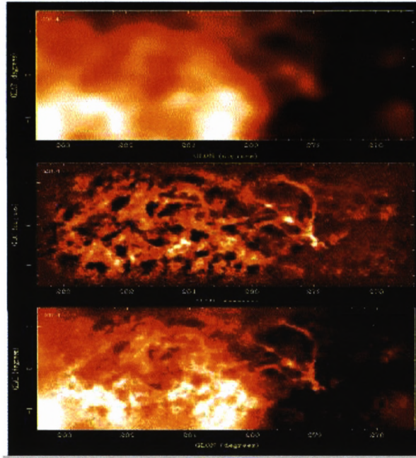
Figure B.20: HI images of the Galactic chimney GSH277+0+36 made with Parkes (top), the ATCA interferometer (middle), and the combined data (bottom) (McClure-Griffiths et al. 2002). Mapping large structures in the Milky Way requires both rapid (and accurate) interferometric mosaics, and supporting single dish data; the E-configuration will provide the one, while the Green Bank Telescope provides the other.
