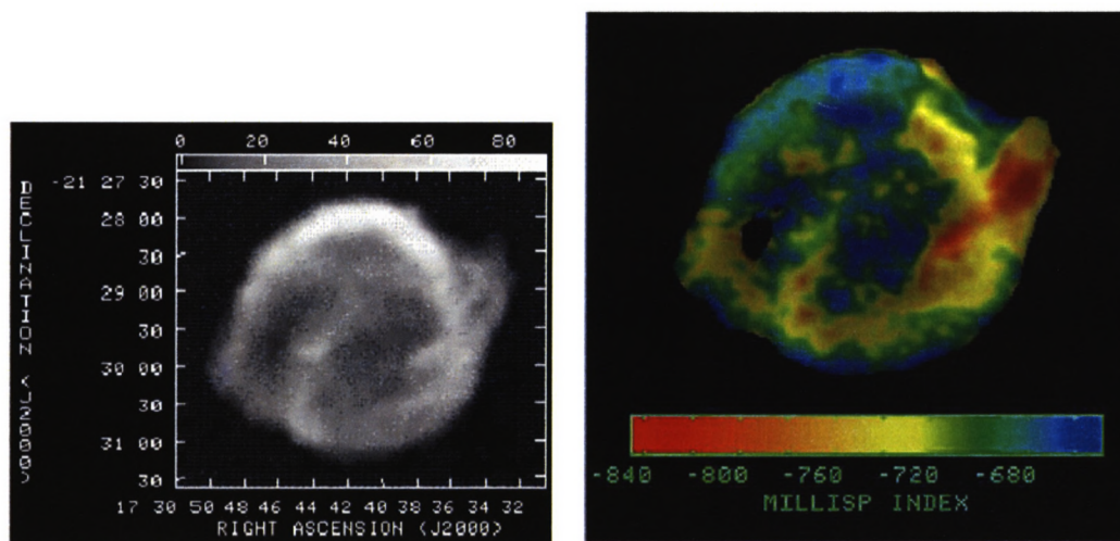
Figure B.30: Kepler's supernova remnant, as observed with the VLA at 1.4 and 5 GHz by Delaney et al. (2002). Left: Total intensity image, at 7'' resolution, showing both the simple circular shell expected in a remnant of this age, and the wisps and filaments which have developed within this structure. Right: a two-frequency spectral index map, showing that flatter and steeper spectral regions correlate with the filamentary structures. Such studies provide information on the nature of particle acceleration sites in the remnant; expanded frequency coverage will enable the study of details of the particle acceleration physics. The improved resolution and continuous frequency coverage of the EVLA will allow this type of study to be carried out on many such objects.
