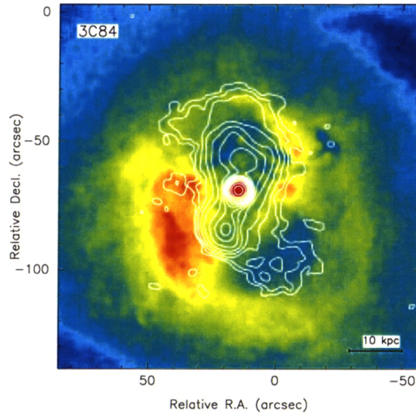
Figure 3.15: The cooling core source 3C84 in the Perseus galaxy cluster: 1.4 GHz (VLA) contours over 0.5–1 keV (Chandra) color image, from Fabian et al. (2000). Note the anti-correlation between the radio lobes and the X-ray emission, and the bright X-ray rims around the radio lobes. These rims are cooler than the surrounding gas, and not the result of shocks; the bubbles themselves may contain hotter gas. The radio-emitting plasma has pushed the X-ray emitting gas aside.
