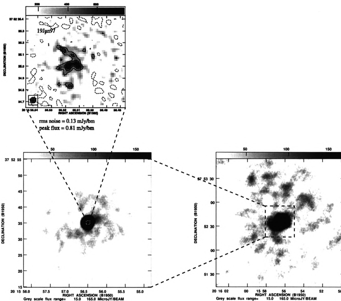
Figure B.12: The thermal wind of the luminous blue variable P Cygni. MERLIN 5 GHz images (top; Exter et al. 2002) show profound variability on timescales as short as a few days, but are severely limited in sensitivity (the peak contour here is 5\sigma ) and resolve out much of the flux density. The VLA images at the same frequency (bottom; made by stacking seven years of monthly VLA monitoring, Skinner et al. 1998) also show very complex structure, on scales ranging from the (sub-arcsecond) resolution, to a few arcminutes. This extended emission is confirmed by comparison with optical images and VLA data taken at 15 GHz, which both show much of the same structure. The New Mexico Array by itself will allow imaging at the MERLIN resolution, with ten times higher sensitivity; the full EVLA will add another factor 10 in sensitivity, and provide incomparably more reliable imaging, of structures covering a much wider range of angular scales. The improved sensitivity will also allow imaging at much higher frequencies, allowing a factor 10 higher spatial resolution. These higher frequencies will also require adding in the short-baseline E-configuration, to allow mosaicing the large-scale structure: the primary beam at 43 GHz is only \sim 1 arcmin FWHM.
