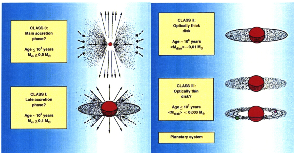
Figure B.4: In the current “standard model” of star formation, young stellar objects (YSOs) are divided into classes based on their spectral energy distributions. In the earliest stage of star formation, where most of the accretion takes place, the emission from Class 0 sources is completely dominated by far infrared emission from cold dust. In all cases the source also hosts a thermal jet, indicating the fundamental role of such outflows in the star formation process. In the next stage, Class I sources are less uniformly surrounded by dust; much of the accreting material is now in the form of a thin disk, and the observed emission is dominated by a combination of that from the star itself, and thermal emission from the disk and residual dust cloud. Class II sources are distinguished by the dominance of the stellar black body and the near disappearance of the dust cloud. Finally, Class III sources host a much less massive (and optically thin) disk, and may start to form planets.
