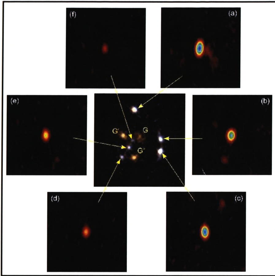
Figure B.29: The gravitational lens system B1359+154, found by the Cosmic Lens All-Sky Survey (CLASS). This composite shows the Hubble Space Telescope optical image, surrounded by six VLBA images of the lens background radio source (Rusin et al. 2001). This is the first arcsecond-scale system in which a source is lensed into more than four detectable images.
