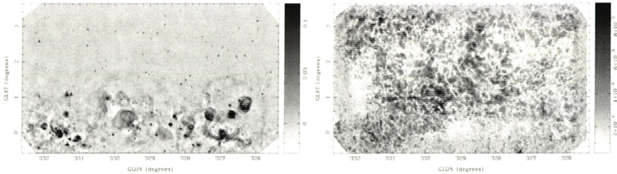
Figure B.19: Diffuse total intensity (left) and linearly polarized (right) Galactic emission (Gaensler et al. 2001). The total intensity illustrates the huge variety of sources in the Galactic plane. Note the almost total lack of correspondence between this and the polarized intensity; the foreground H II regions block the polarized signal, but the connection between the other sources and these structures is far from obvious.
