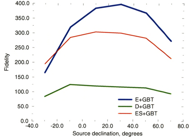
Figure 5.10: The fidelity of the proposed E-configuration compared to the existing D-configuration, with the southern-extended ES-configuration added. For all simulations, GBT data have been added. The simulation is of an object whose size is six times the antenna primary beamwidth, taken in a single 7 X 7 raster. The fidelity is defined as the ratio between the peak brightness in the model image to the rms of the difference between the model and reconstructed image.
