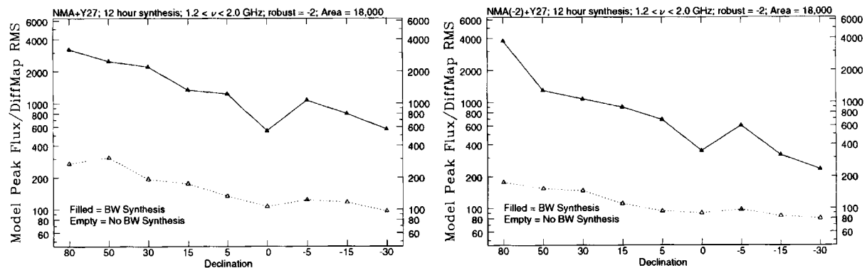
Figure 5.5: The effect on imaging fidelity of the EVLA by reducing the number of New Mexico Array antennas from ten to eight. The left panel shows the full EVLA, the right panel shows the EVLA minus two antennas. The antennas removed are at Pietown and Vaughn. The loss of fidelity is typically a factor of two to three, and worsens with decreasing declination.
