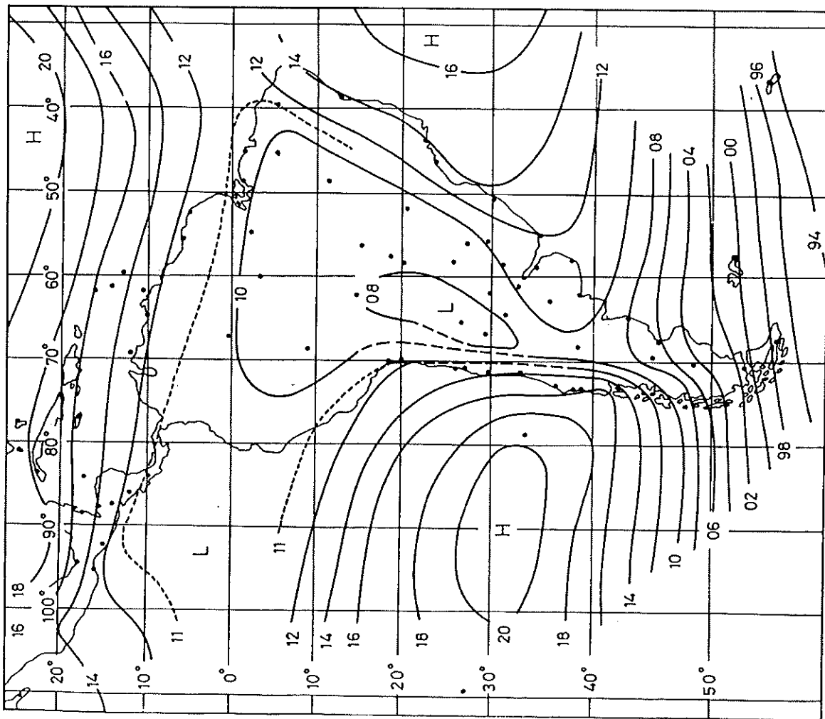
Fig. 1. Atmospheric pressure at sea level, average of the three months December-February (southern summer). 20 = 1,020 mbar.
