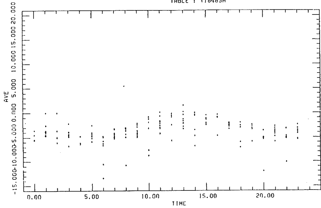
DIURNAL AIR TEMPERATURE VARIATION
