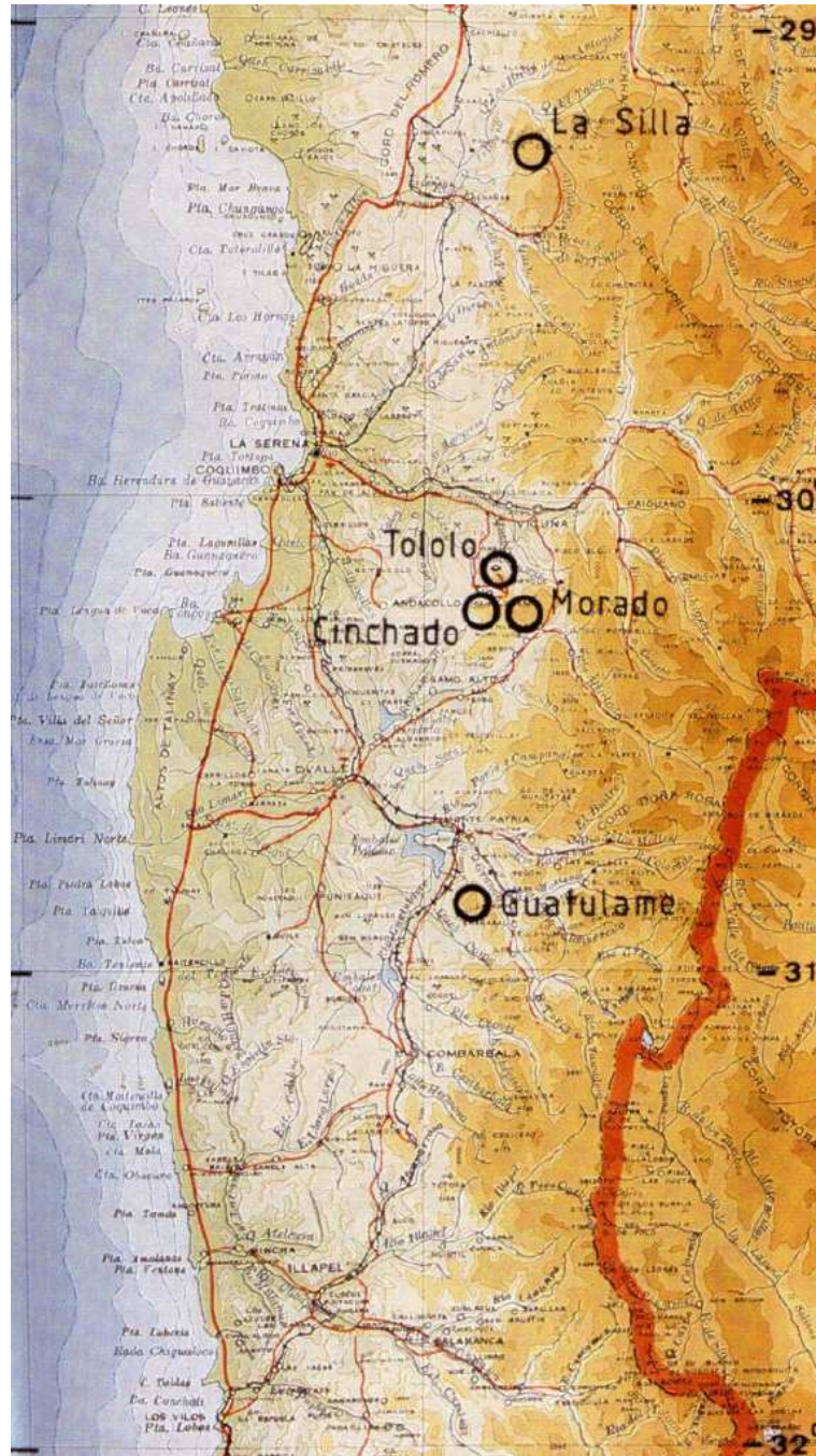
Figure 50: This map shows the mountains that played a role in ESO's search for a site (taken from A. Blaauw's book: "ESO's Early History").
