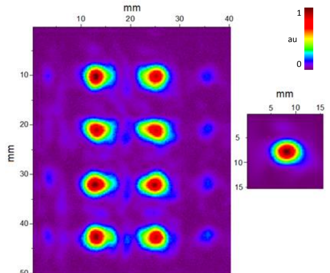
Fig. 1. The measured 8-beam pattern (left) and the incident beam on the same plane when the grating is replaced with a flat mirror (right). The color indicates the intensity.
